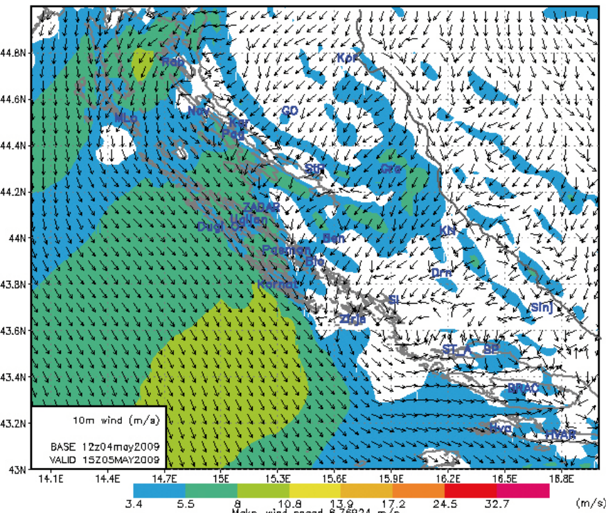
2km Maslenica 10m mean wind at 15Z05MAY2009 UTC 27hrs forecast
