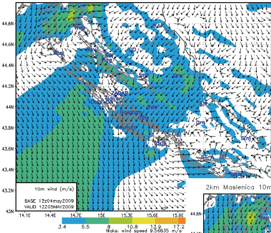
2km Maslenica 10m mean wind at 12Z05MAY2009 UTC 24hrs forecast
